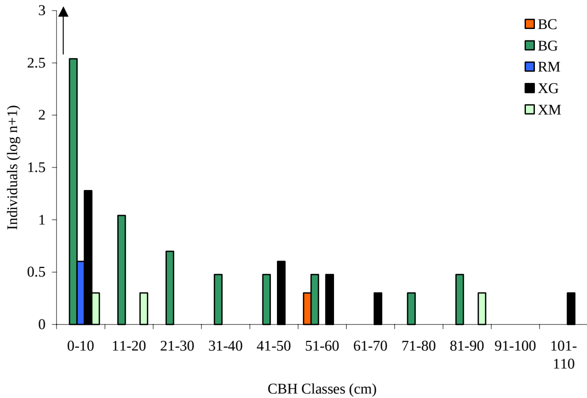
Figure 3.12: Species CBH Classes (log n+1)
