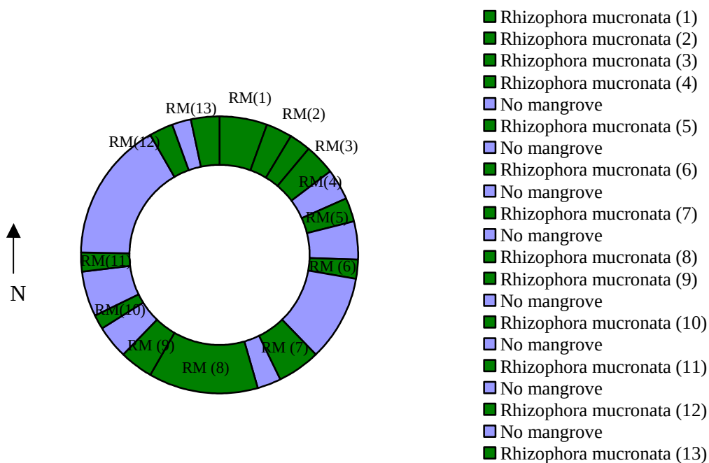
Figure 3.9: Dominant Mangrove Stands Lagoon 3
